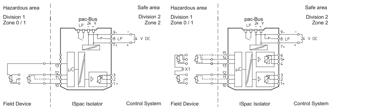
9180/1.-77-11 connection diagram
